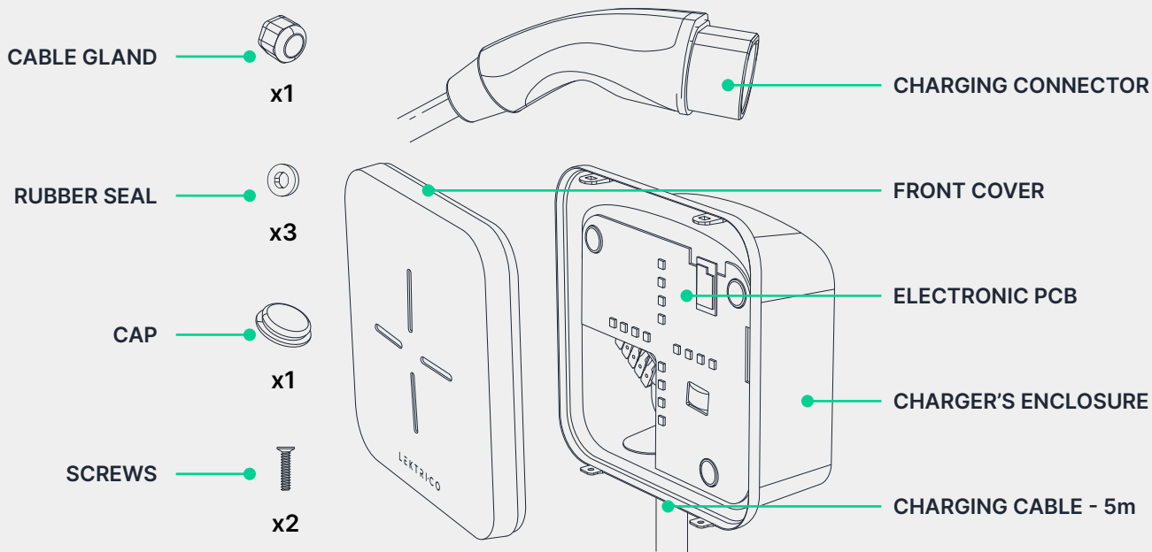
Fig. 1 - Main components of the ONE™ charger
