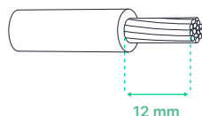
Fig. 7 - Insulation stripping length.
