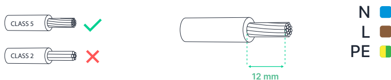
Fig. 7 - Insulation stripping length.
